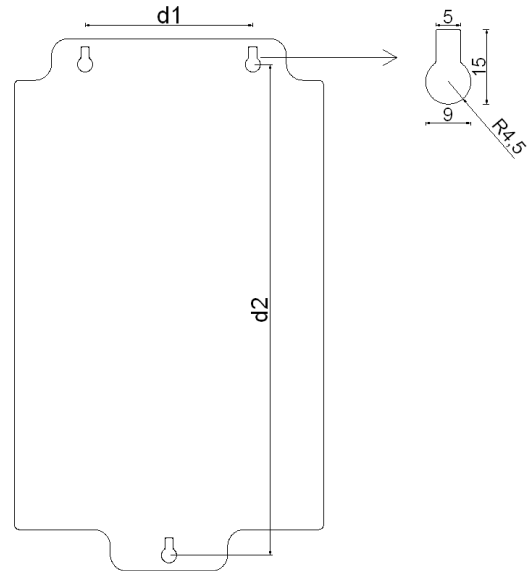
Figure 2.2 Mounting Holes
