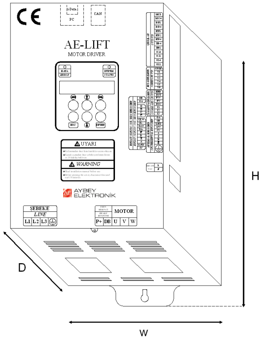
Figure 2.1 Device Box
